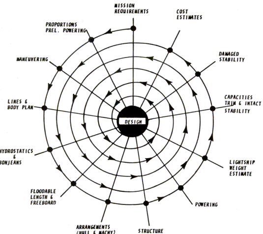
Figure 6 Maneuverability should be an important spoke in the "Ship Design Spiral." [25]
