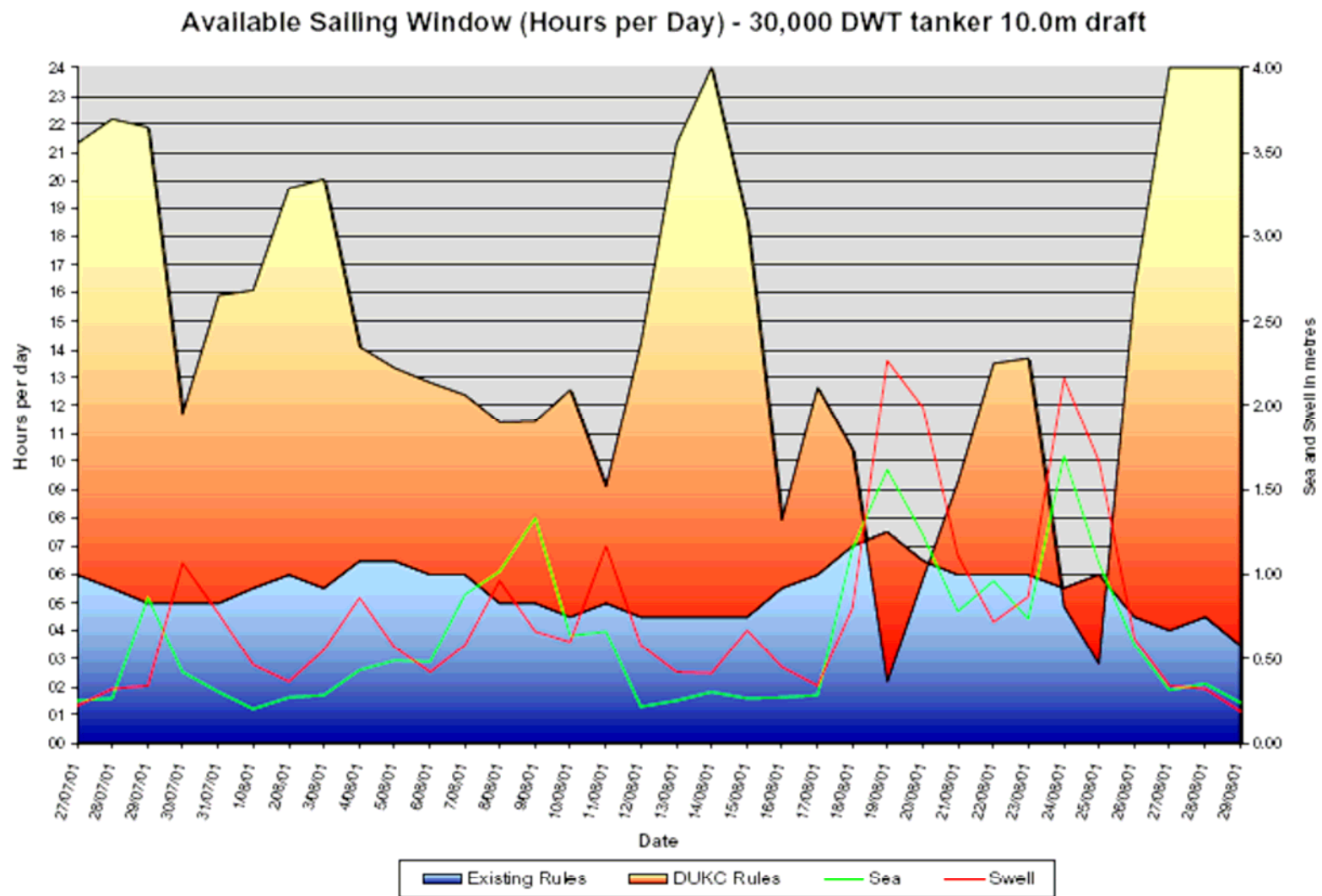
Figure 5 Graph comparing operating windows allowed by the static underkeel clearance rule and the application of DUKC at Port Taranaki. Note the correlation with swell height and the non-conservative situations with the static rule on the 19 th and 25 th of August 2001 (Ref. 3).
