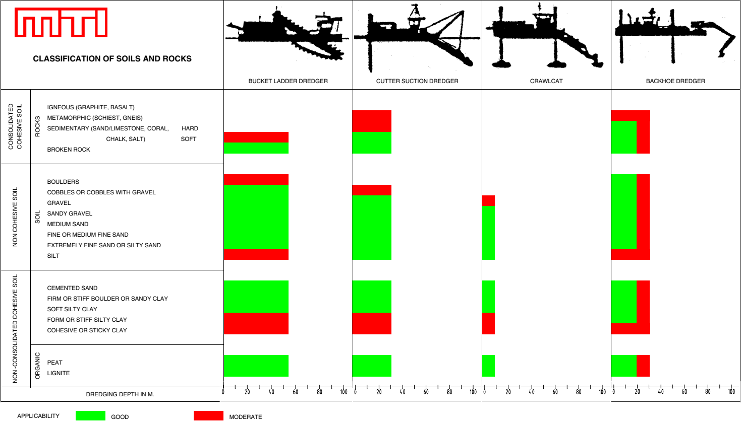
DREDGING EQUIPMENT AND APPLICABILITY
